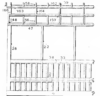
Fig. 5657. Part Elevation of Side Framing.
